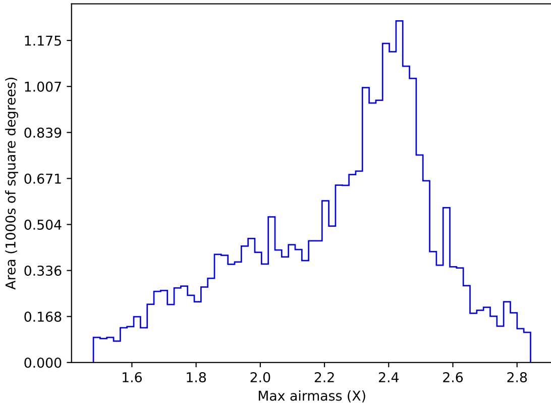
ddf_loaded_fl4_v3.4_10yrs All sky r band: Max airmass
