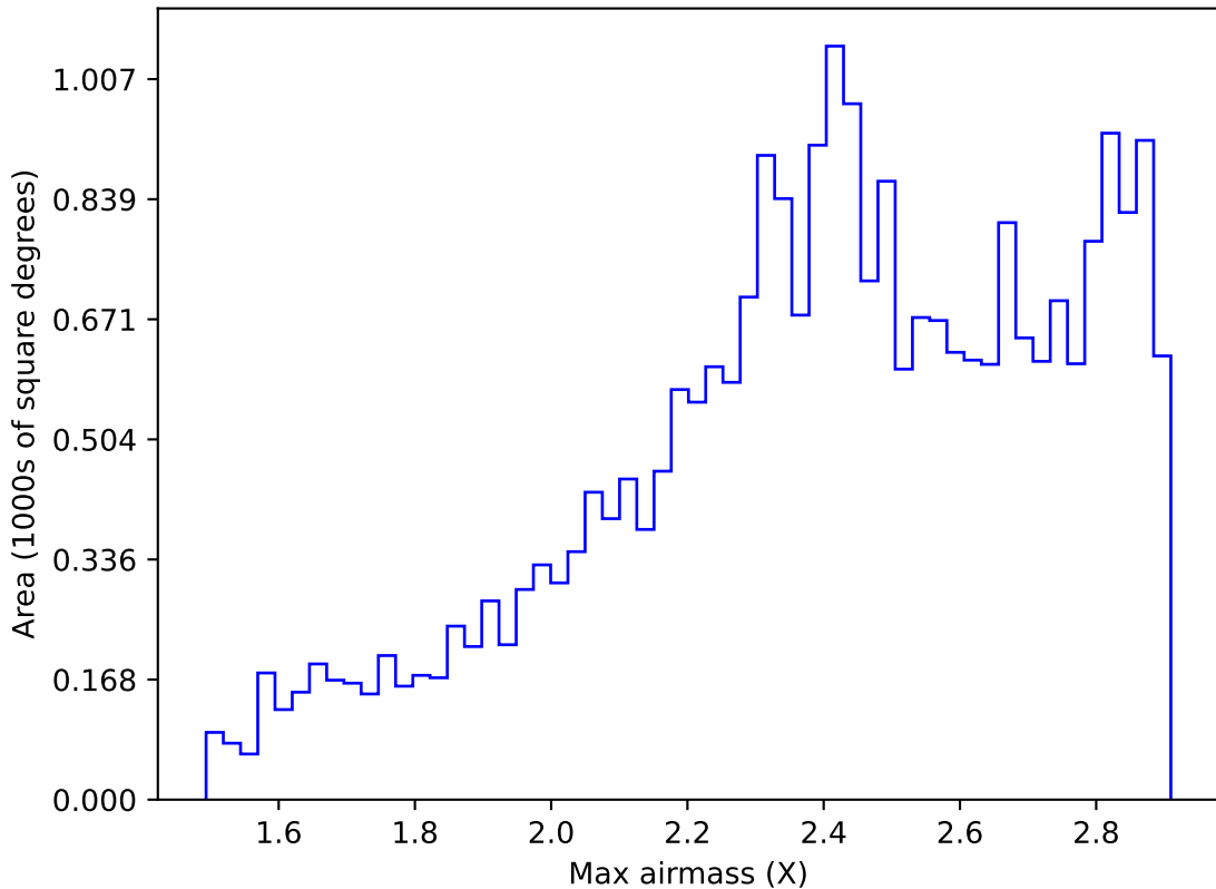
ddf_loaded_fl4_v3.4_10yrs All sky i band: Max airmass
