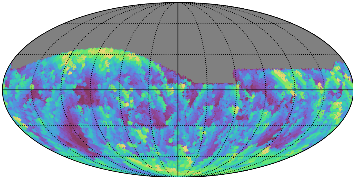
ddf_loaded_fl4_v3.4_10yrs All sky g band: Max airmass
