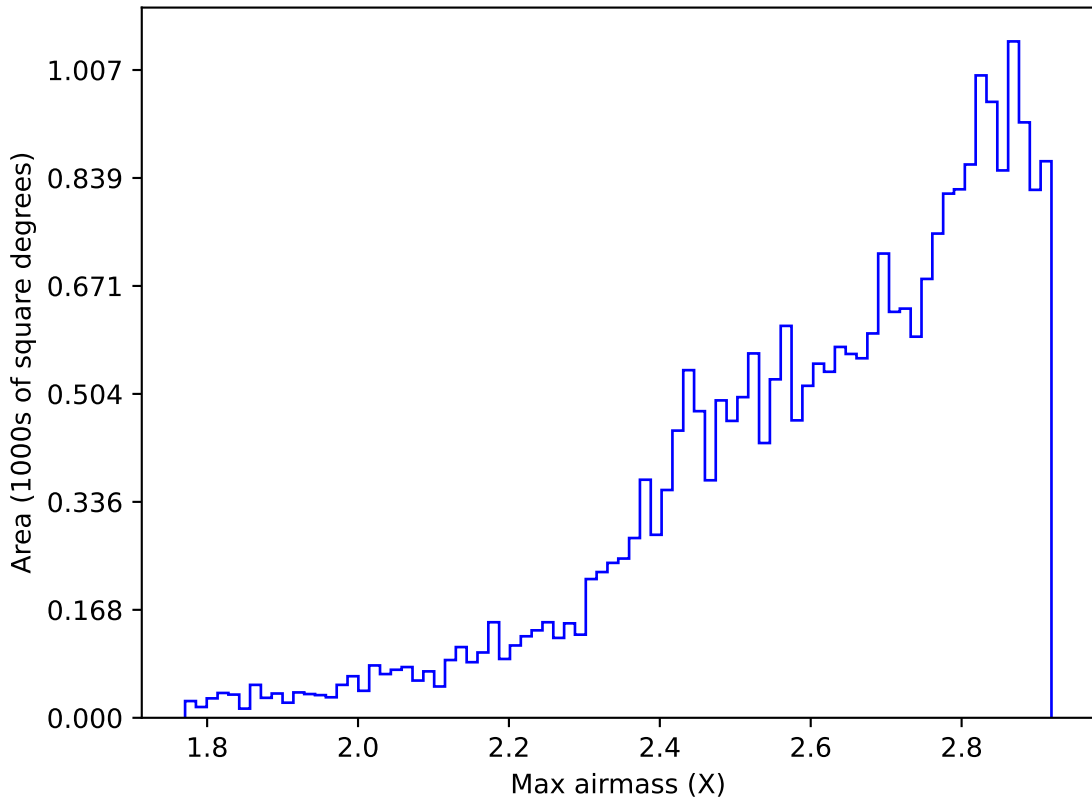
ddf_loaded_fl4_v3.4_10yrs All sky all bands: Max airmass
