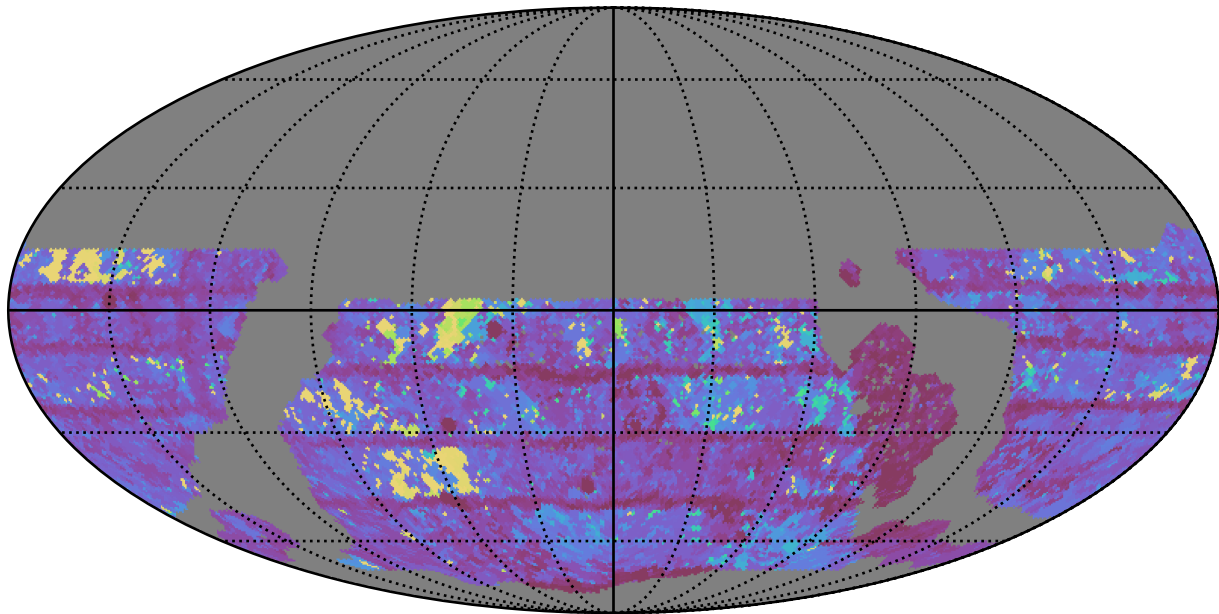
ddf_loaded_fl4_v3.4_10yrs WFD z band: Max Inter-Night Gap
