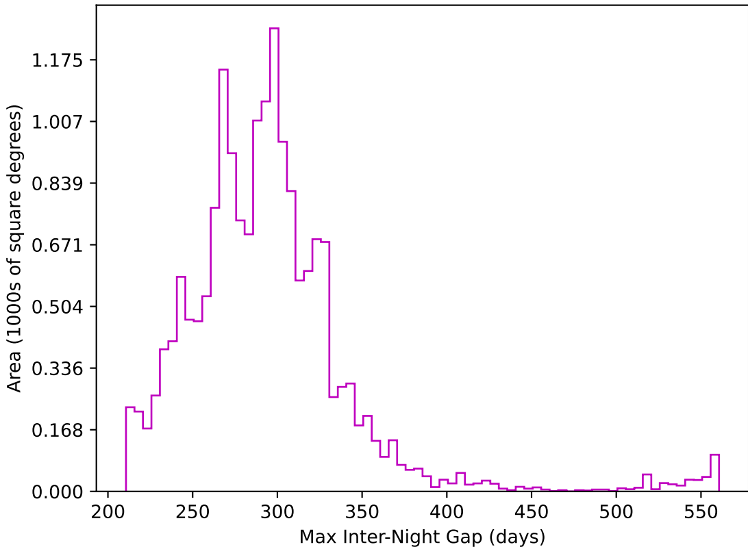
ddf_loaded_fl4_v3.4_10yrs WFD z band: Max Inter-Night Gap
