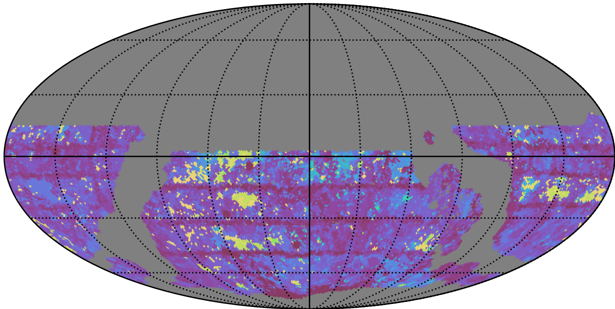
ddf_loaded_fl4_v3.4_10yrs WFD y band: Max Inter-Night Gap
