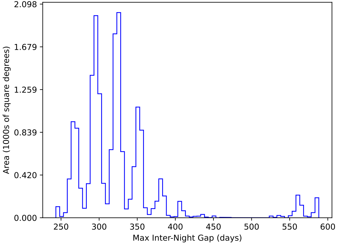
ddf_loaded_fl4_v3.4_10yrs WFD y band: Max Inter-Night Gap
