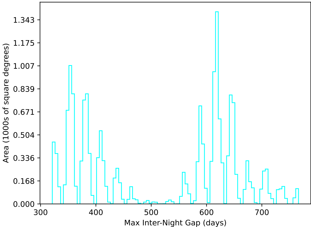
ddf_loaded_fl4_v3.4_10yrs WFD u band: Max Inter-Night Gap
