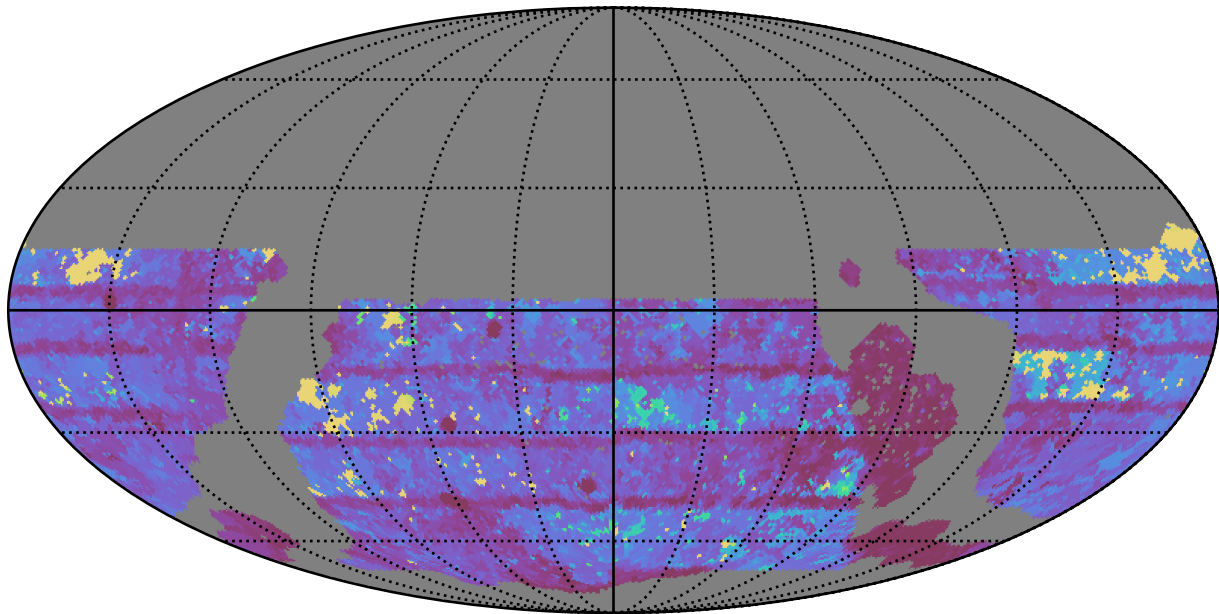
ddf_loaded_fl4_v3.4_10yrs WFD r band: Max Inter-Night Gap
