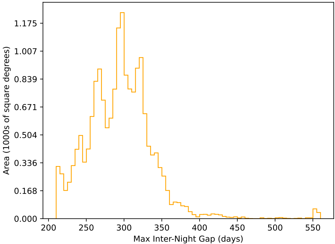
ddf_loaded_fl4_v3.4_10yrs WFD r band: Max Inter-Night Gap
