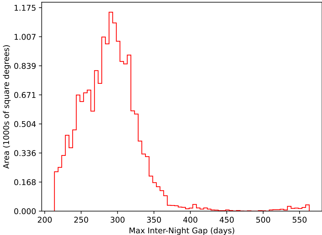
ddf_loaded_fl4_v3.4_10yrs WFD i band: Max Inter-Night Gap
