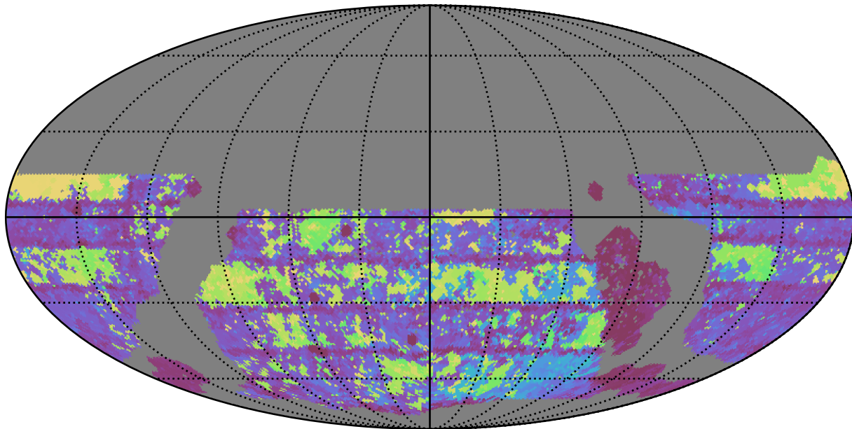
ddf_loaded_fl4_v3.4_10yrs WFD g band: Max Inter-Night Gap
