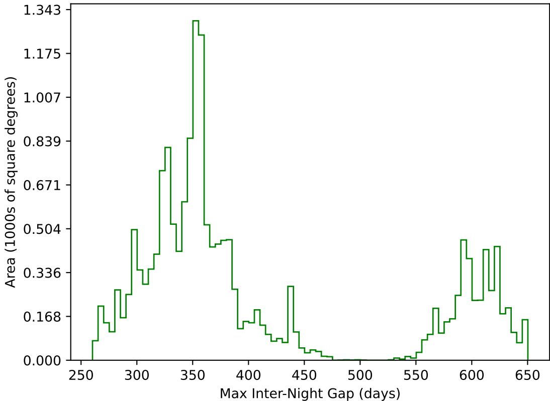
ddf_loaded_fl4_v3.4_10yrs WFD g band: Max Inter-Night Gap
