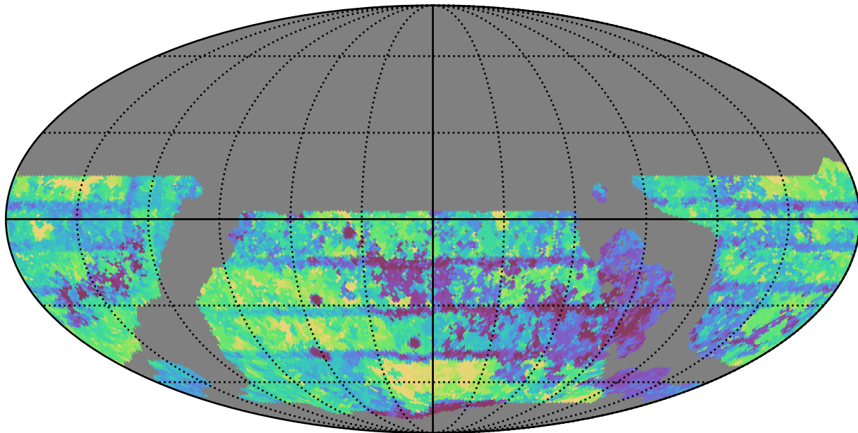
ddf_loaded_fl4_v3.4_10yrs WFD all bands: Max Inter-Night Gap
