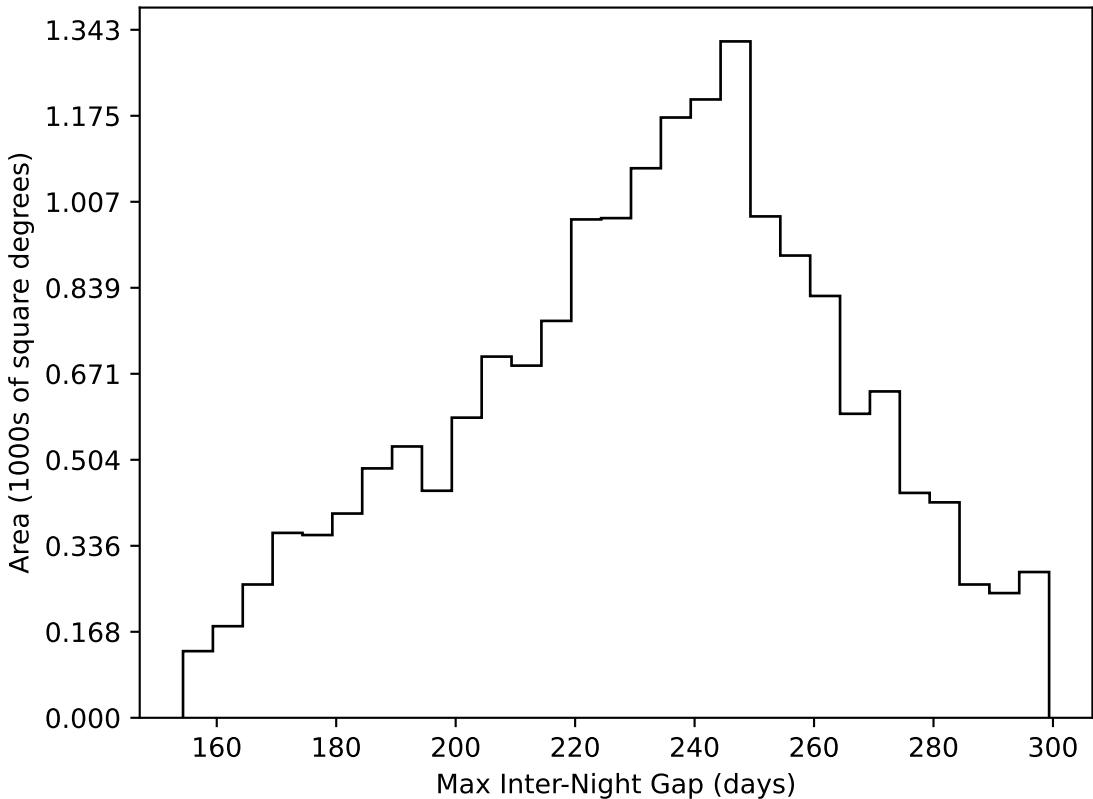
ddf_loaded_fl4_v3.4_10yrs WFD all bands: Max Inter-Night Gap
