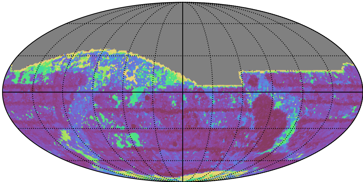
ddf_loaded_fl4_v3.4_10yrs All sky z band: Max Inter-Night Gap
