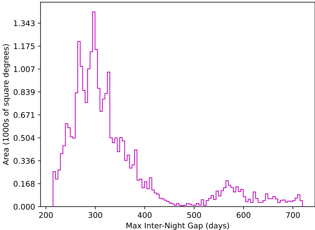
ddf_loaded_fl4_v3.4_10yrs All sky z band: Max Inter-Night Gap
