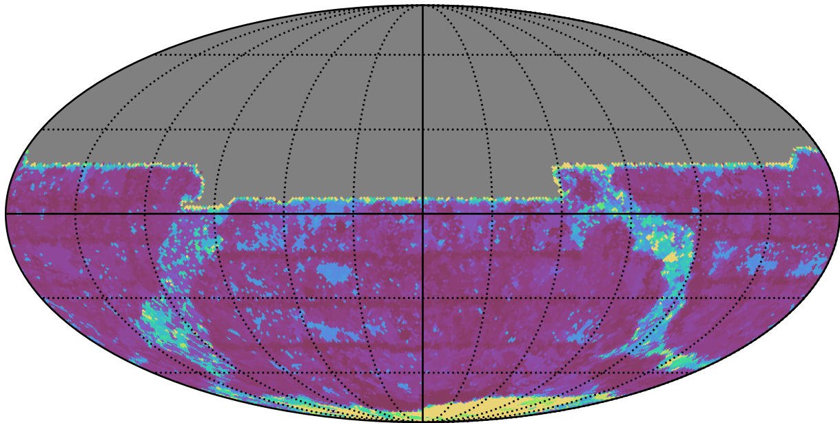
ddf_loaded_fl4_v3.4_10yrs All sky y band: Max Inter-Night Gap
