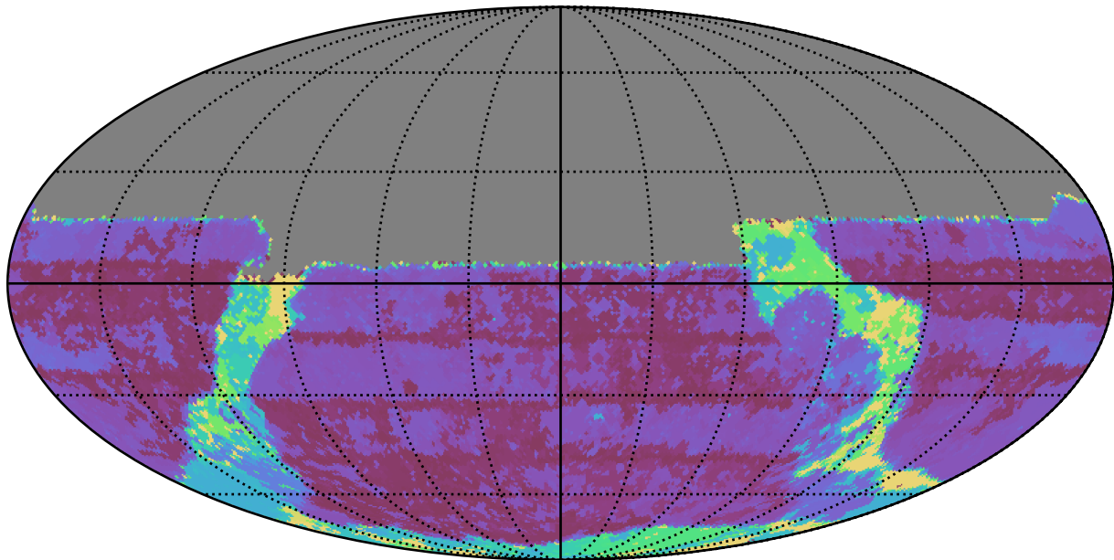
ddf_loaded_fl4_v3.4_10yrs All sky u band: Max Inter-Night Gap
