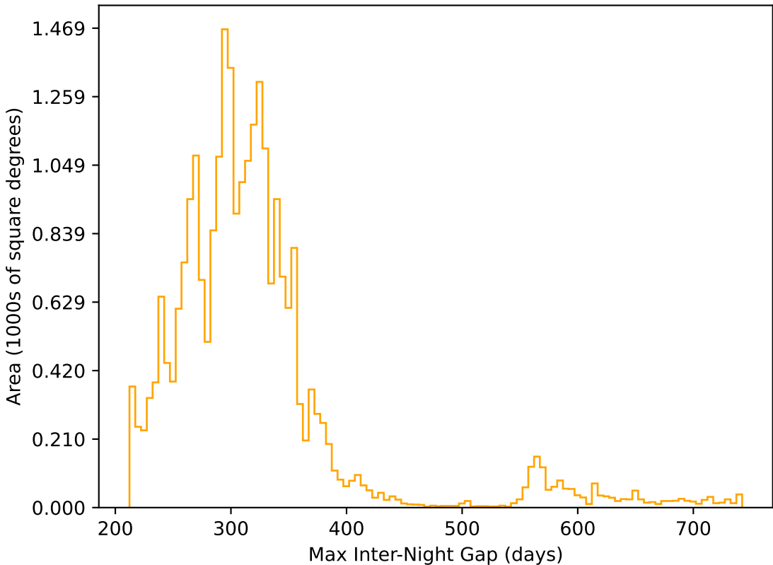
ddf_loaded_fl4_v3.4_10yrs All sky r band: Max Inter-Night Gap
