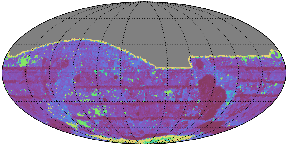
ddf_loaded_fl4_v3.4_10yrs All sky i band: Max Inter-Night Gap
