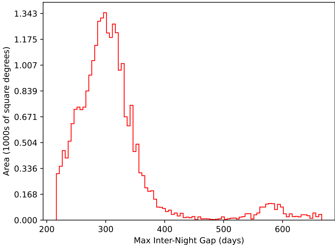
ddf_loaded_fl4_v3.4_10yrs All sky i band: Max Inter-Night Gap
