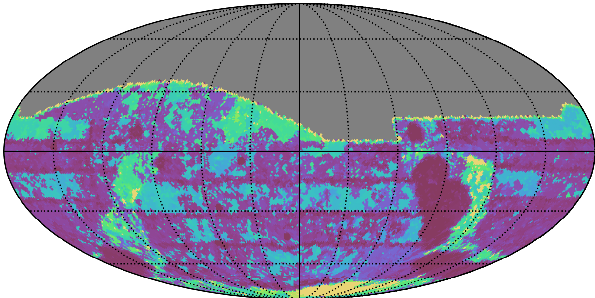
ddf_loaded_fl4_v3.4_10yrs All sky g band: Max Inter-Night Gap
