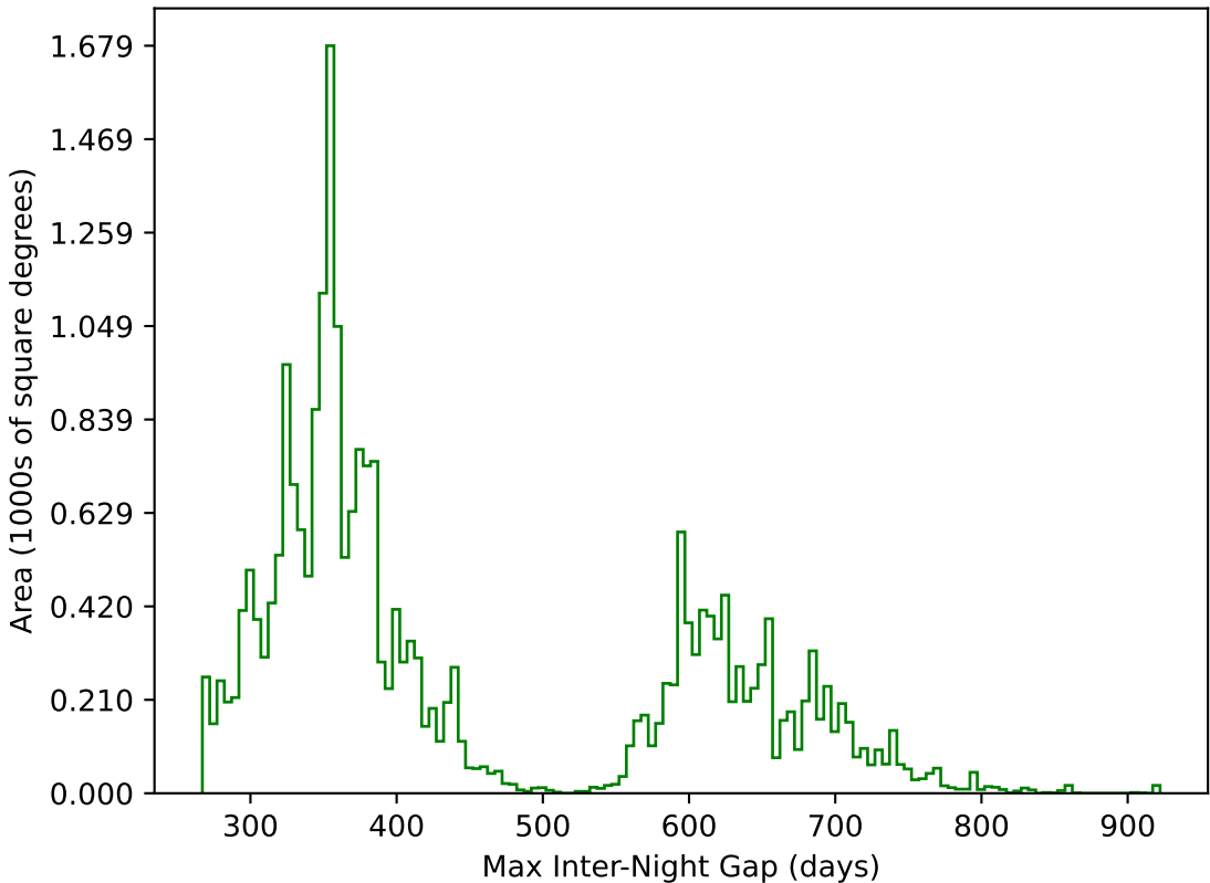
ddf_loaded_fl4_v3.4_10yrs All sky g band: Max Inter-Night Gap
