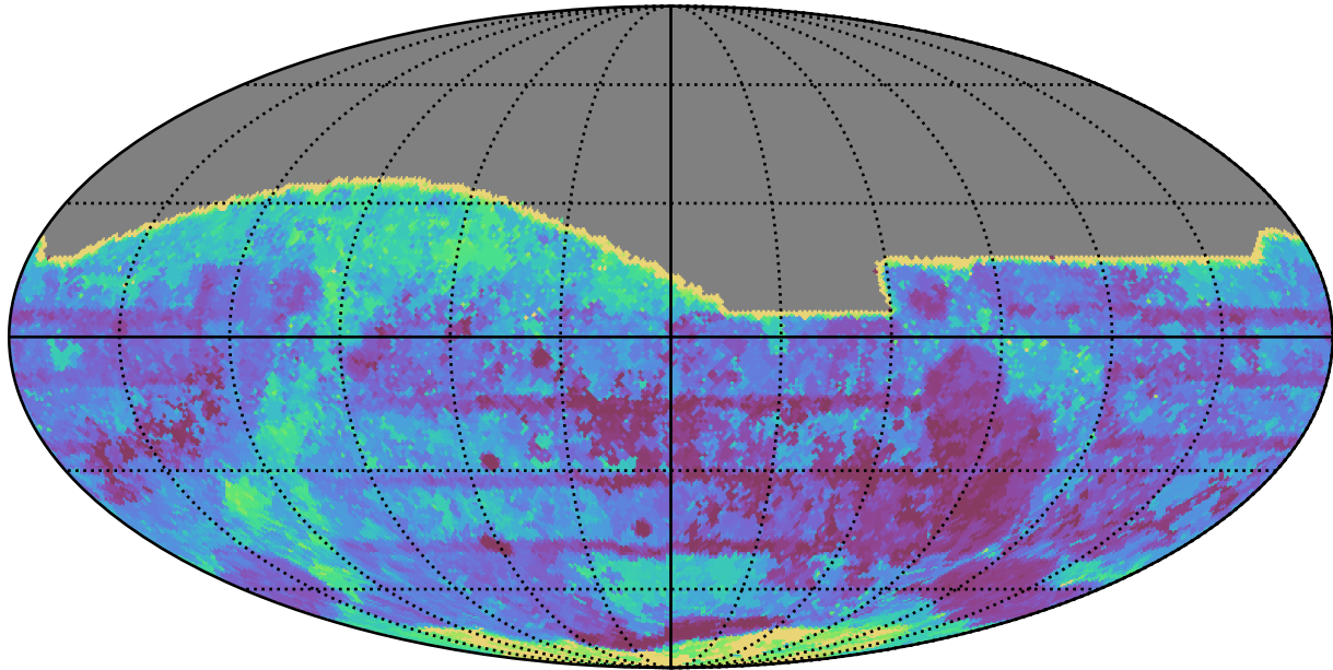
ddf_loaded_fl4_v3.4_10yrs All sky all bands: Max Inter-Night Gap
