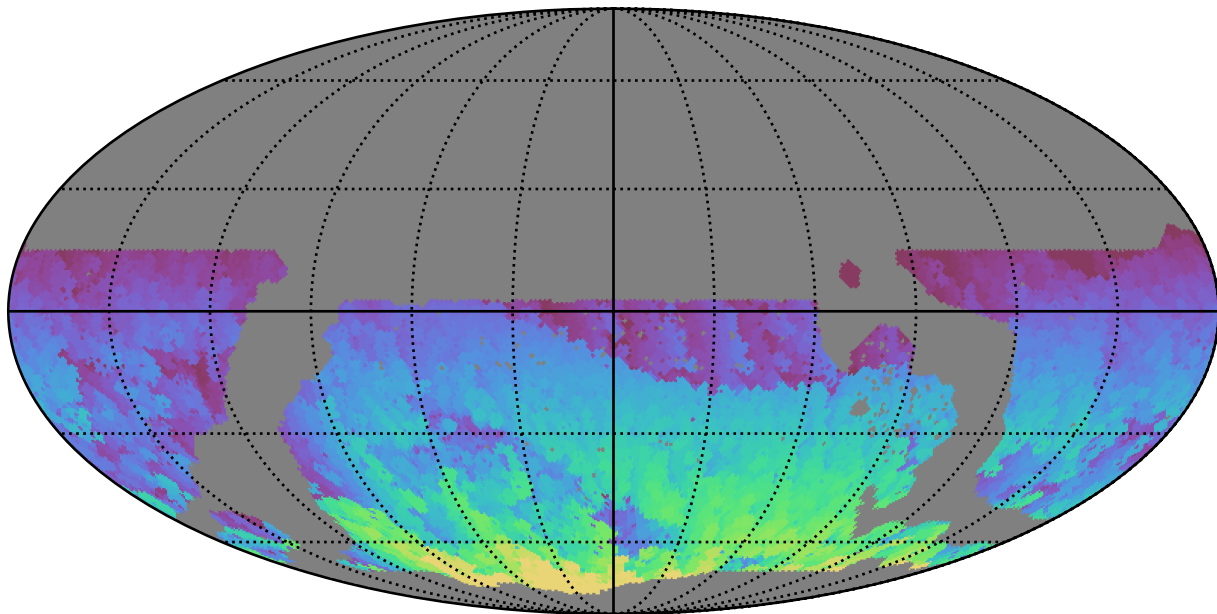
ddf_loaded_fl4_v3.4_10yrs WFD z band: Max HA
