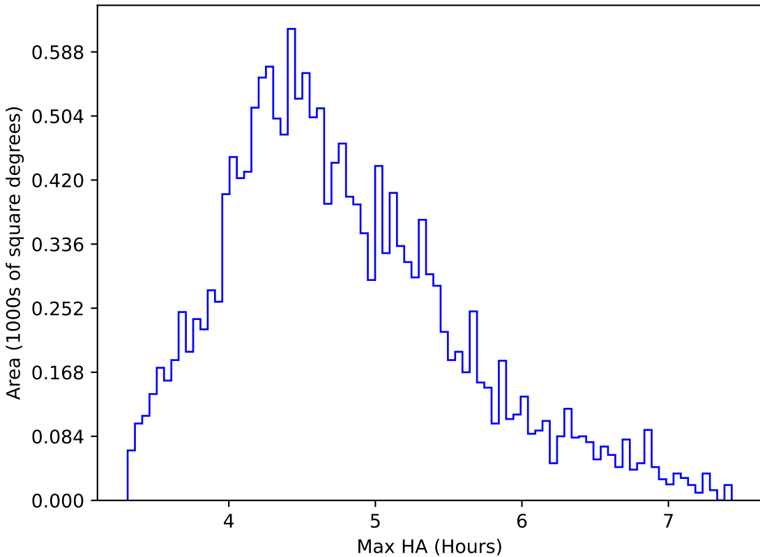
ddf_loaded_fl4_v3.4_10yrs WFD y band: Max HA
