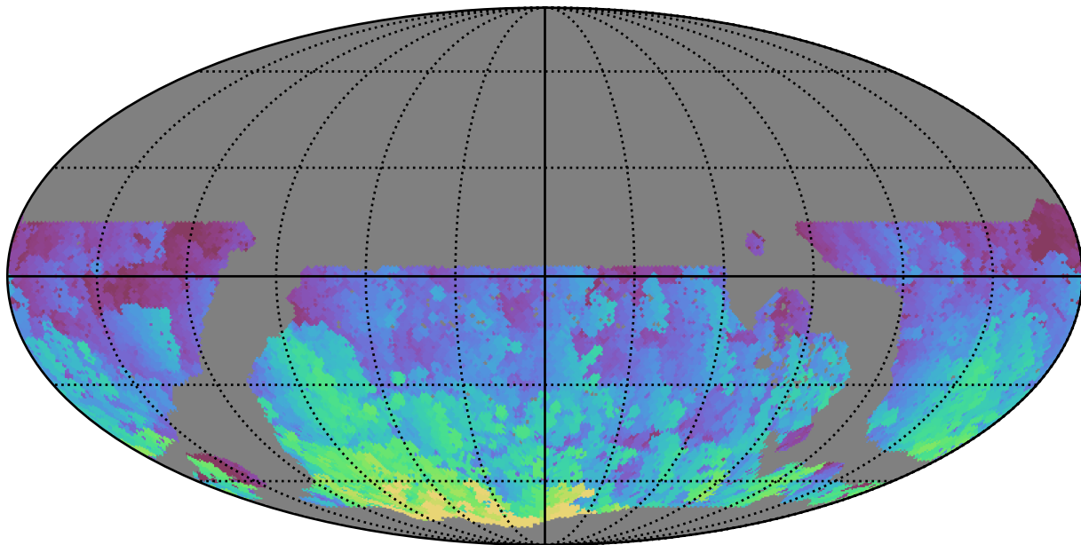
ddf_loaded_fl4_v3.4_10yrs WFD u band: Max HA
