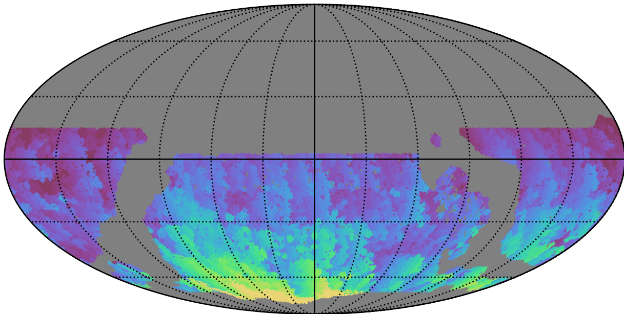
ddf_loaded_fl4_v3.4_10yrs WFD r band: Max HA
