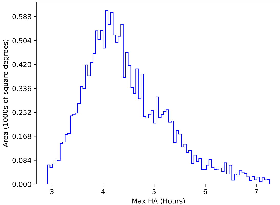
ddf_loaded_fl4_v3.4_10yrs WFD r band: Max HA
