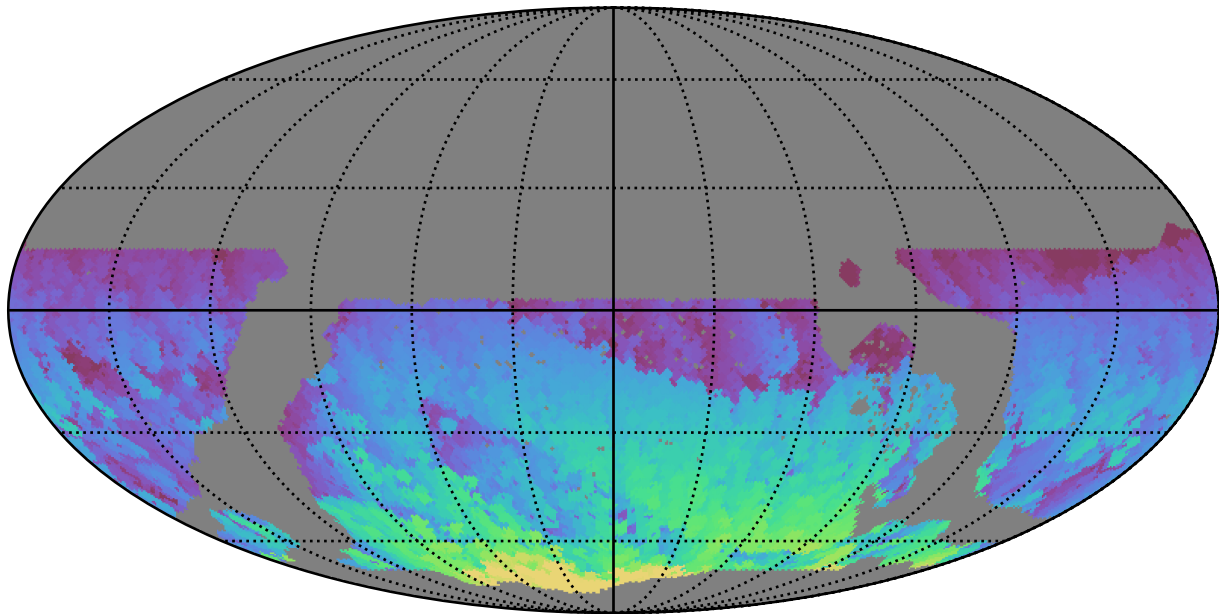
ddf_loaded_fl4_v3.4_10yrs WFD i band: Max HA
