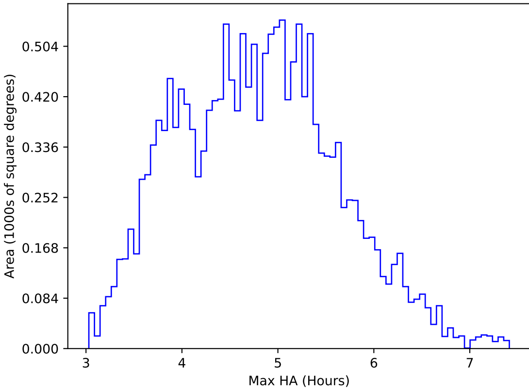
ddf_loaded_fl4_v3.4_10yrs WFD i band: Max HA
