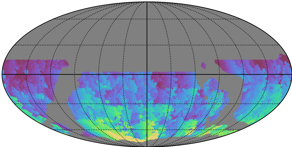
ddf_loaded_fl4_v3.4_10yrs WFD g band: Max HA
