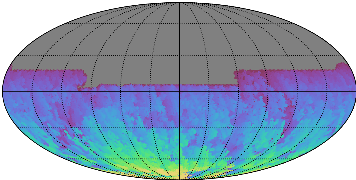
ddf_loaded_fl4_v3.4_10yrs All sky y band: Max HA
