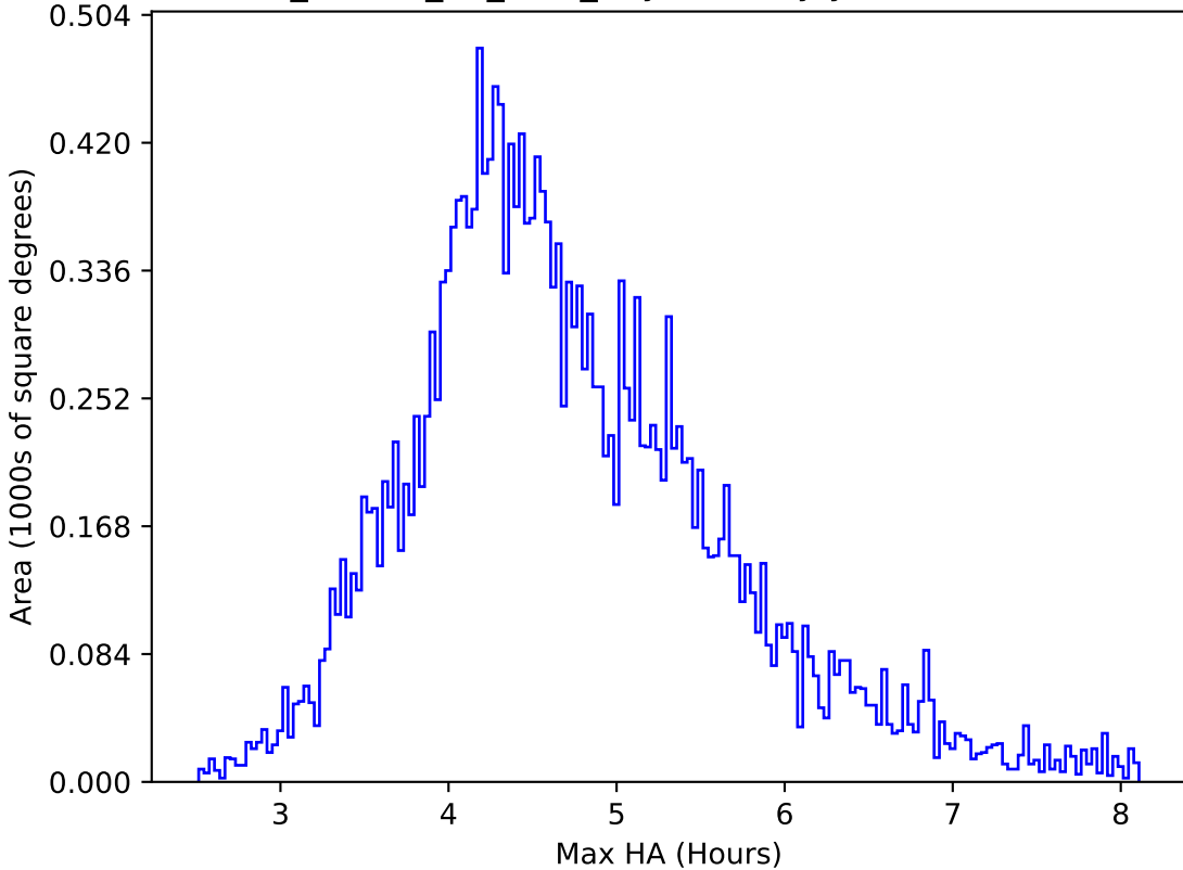
ddf_loaded_fl4_v3.4_10yrs All sky y band: Max HA
