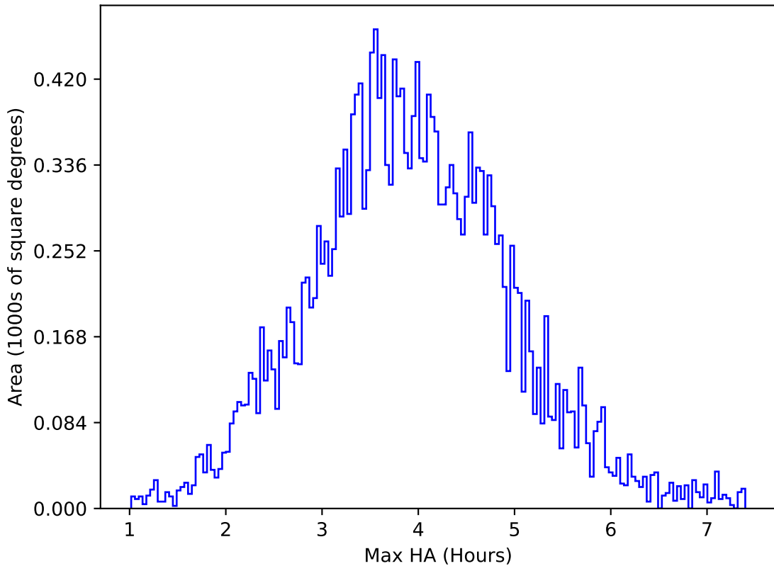
ddf_loaded_fl4_v3.4_10yrs All sky u band: Max HA
