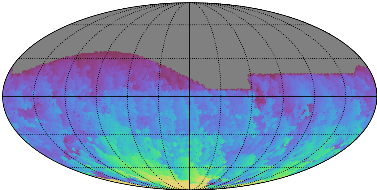
ddf_loaded_fl4_v3.4_10yrs All sky r band: Max HA
