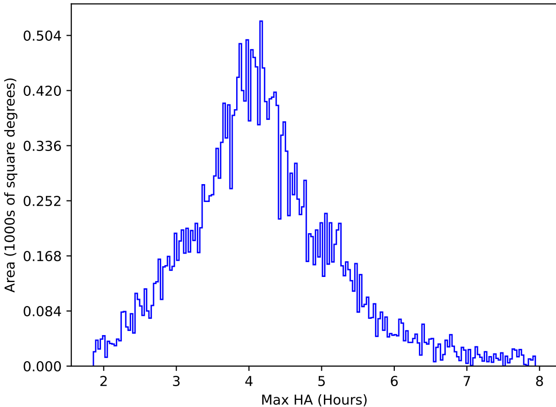
ddf_loaded_fl4_v3.4_10yrs All sky r band: Max HA
