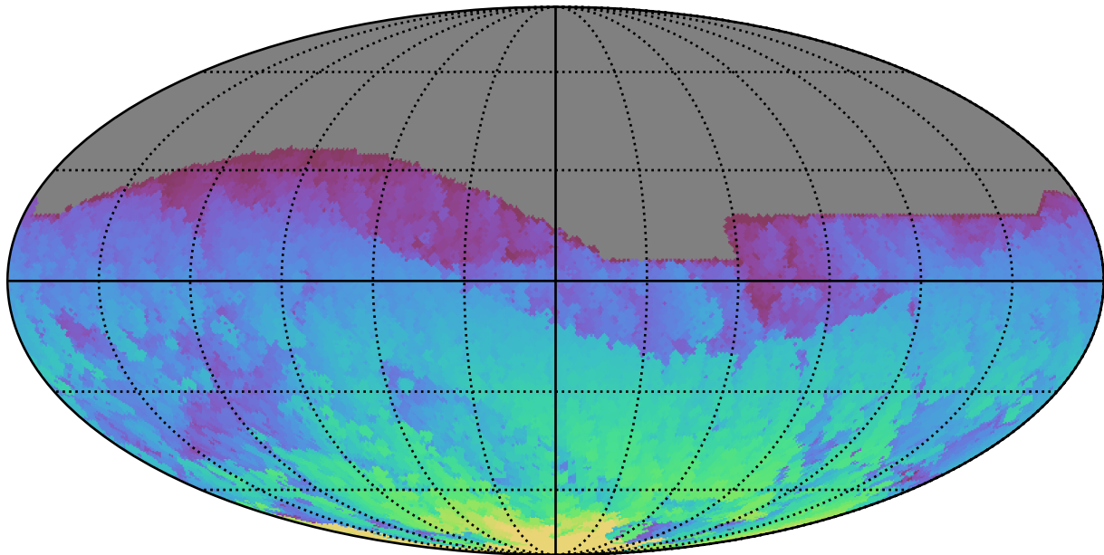
ddf_loaded_fl4_v3.4_10yrs All sky i band: Max HA
