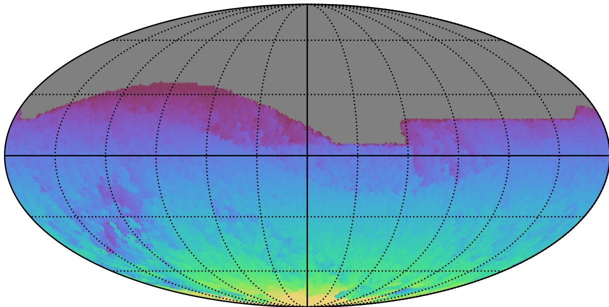
ddf_loaded_fl4_v3.4_10yrs All sky all bands: Max HA
