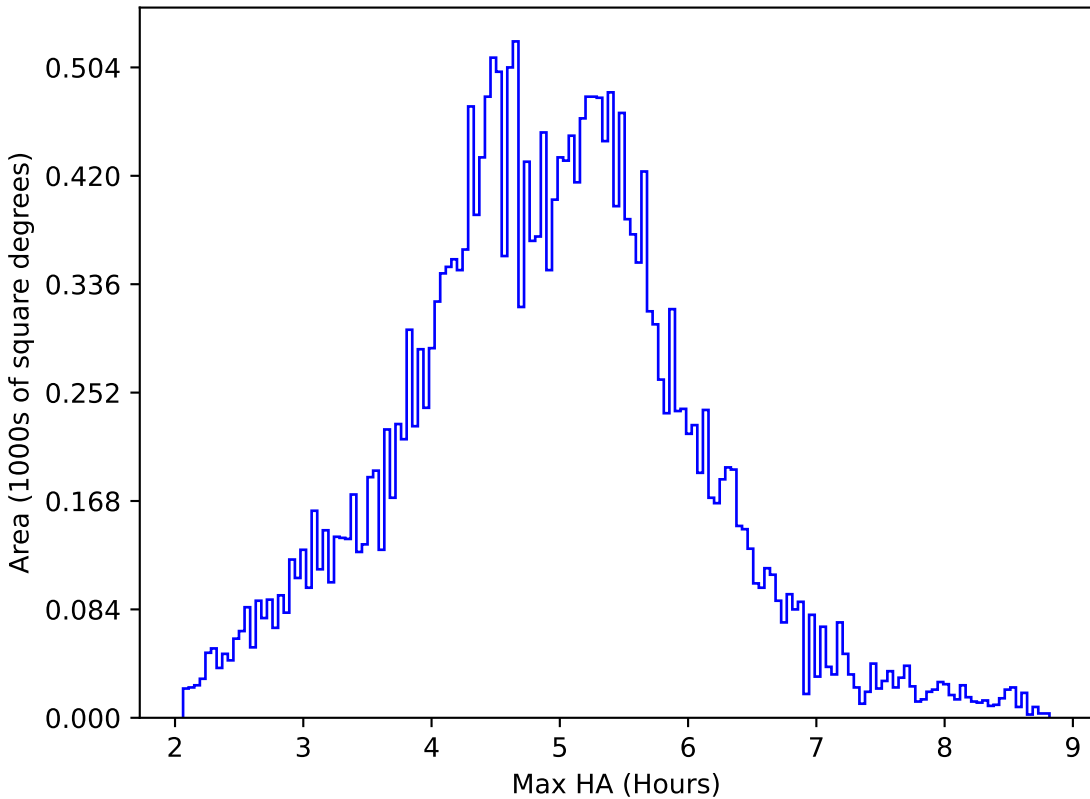
ddf_loaded_fl4_v3.4_10yrs All sky all bands: Max HA
