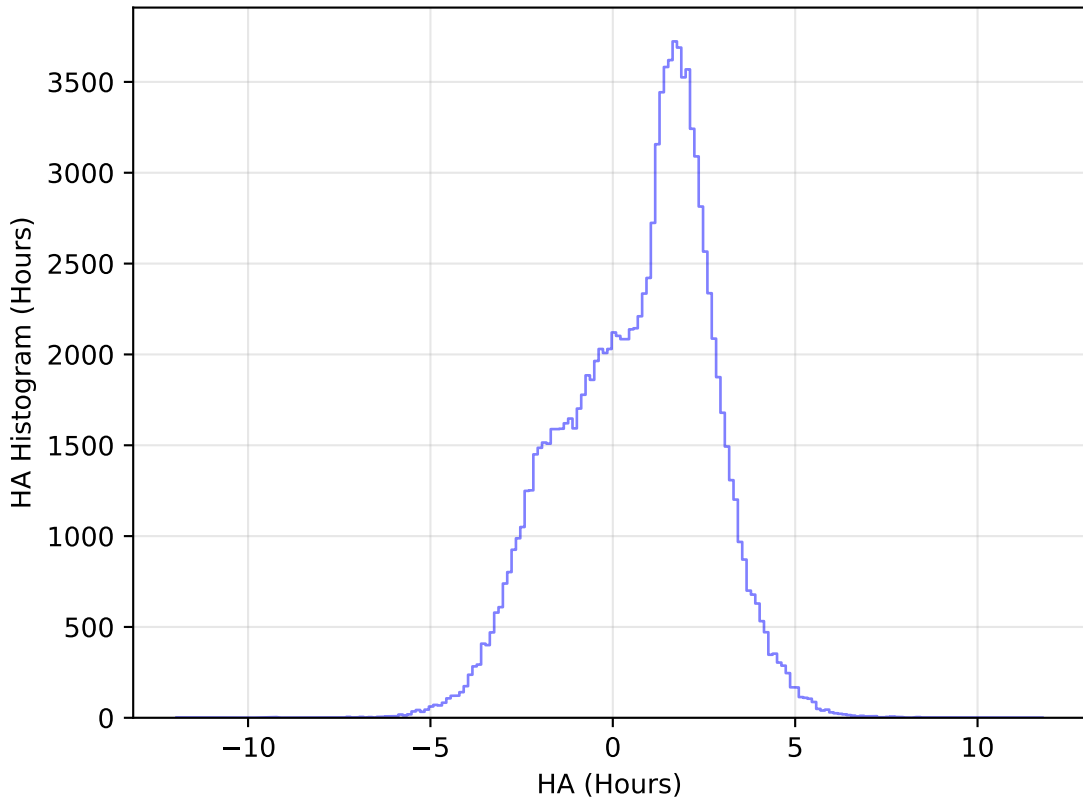
ddf_loaded_fl4_v3.4_10yrs WFD u band: HA Histogram
