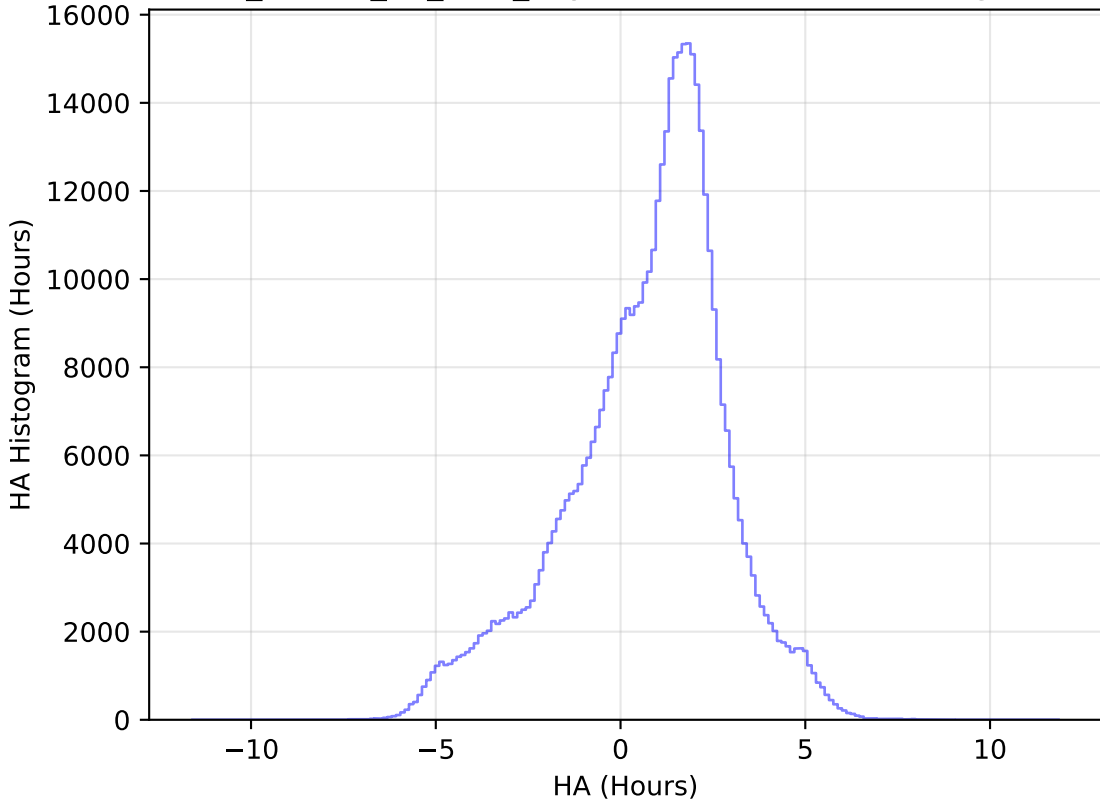
ddf_loaded_fl4_v3.4_10yrs WFD i band: HA Histogram
