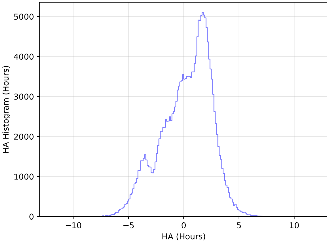
ddf_loaded_fl4_v3.4_10yrs WFD g band: HA Histogram
