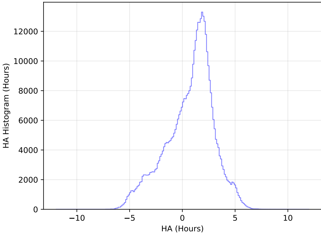
ddf_loaded_fl4_v3.4_10yrs All sky z band: HA Histogram
