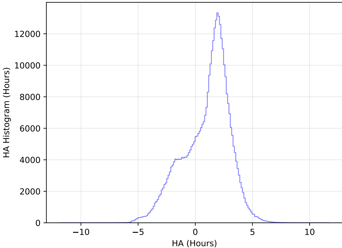
ddf_loaded_fl4_v3.4_10yrs All sky y band: HA Histogram
