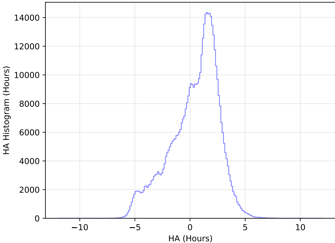
ddf_loaded_fl4_v3.4_10yrs All sky r band: HA Histogram
