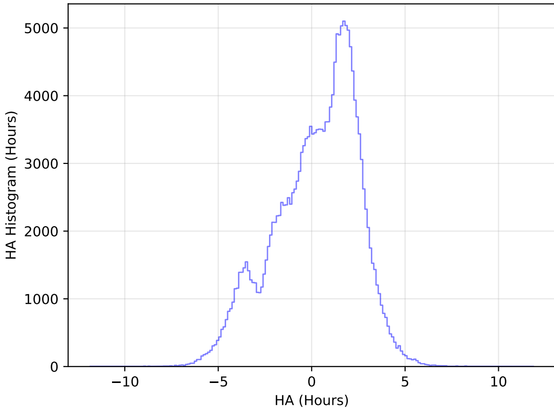
ddf_loaded_fl4_v3.4_10yrs All sky g band: HA Histogram
