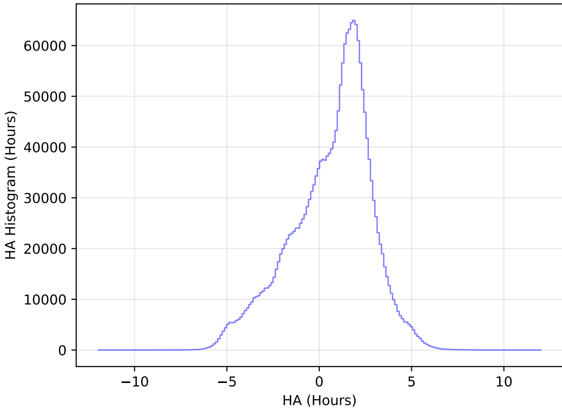
ddf_loaded_fl4_v3.4_10yrs All sky all bands: HA Histogram
